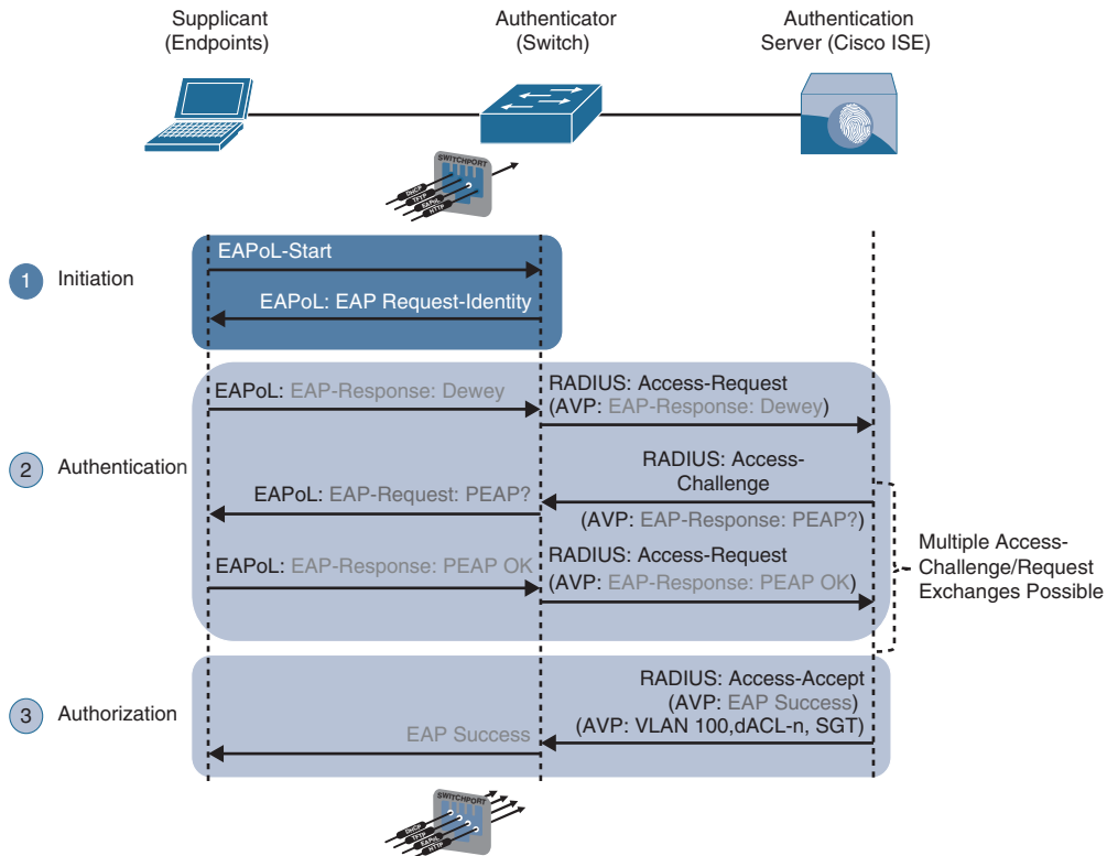
Figure 25-7 Successful 802.1x Authentication Process Flow
