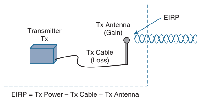
Figure 17-20 Calculating EIRP
