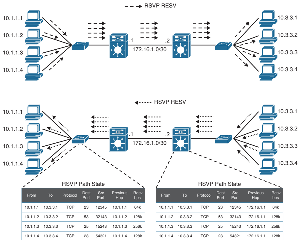
Figure 14-1 RSVP Reservation Establishment
