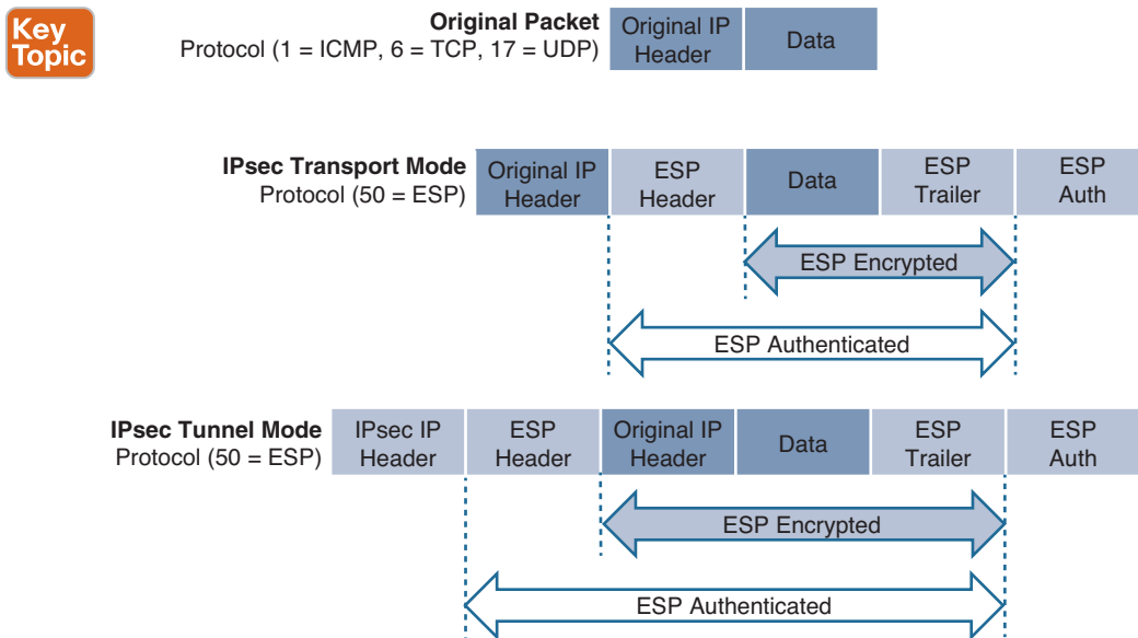
Figure 16-3 IPsec Transport and Tunnel Encapsulation
