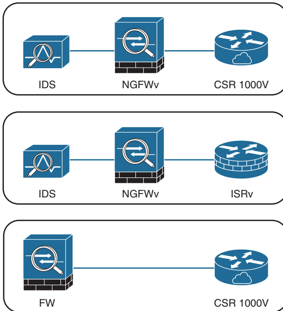
Figure 27-8 Service Chaining
