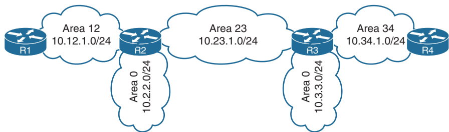
Figure 9-12 Discontiguous Network
