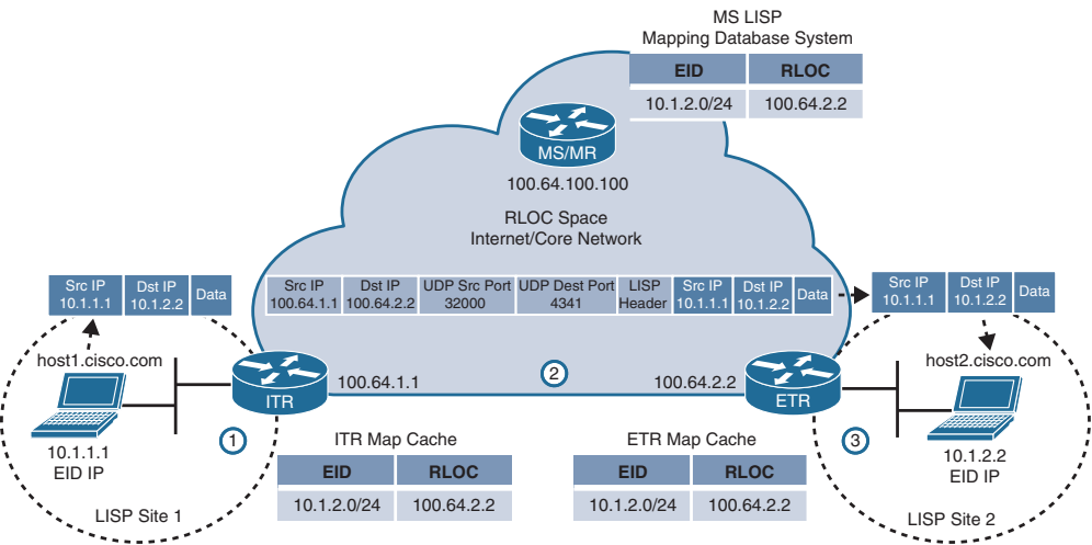
Figure 16-10 LISP Data Path
