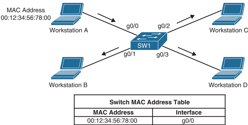
Figure 13-8 Unknown Frame Flooding
