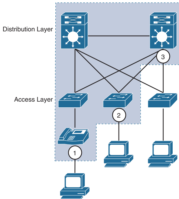
Figure 14-7 Trust Boundaries
