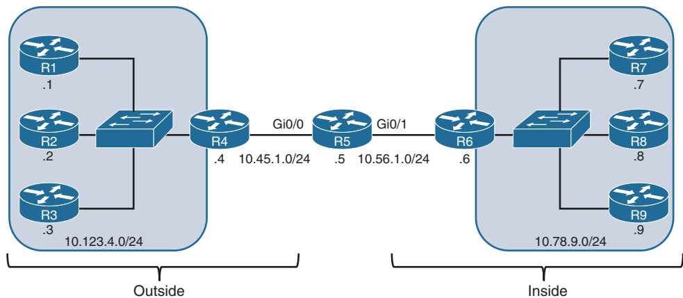
Figure 15-7 NAT Topology
