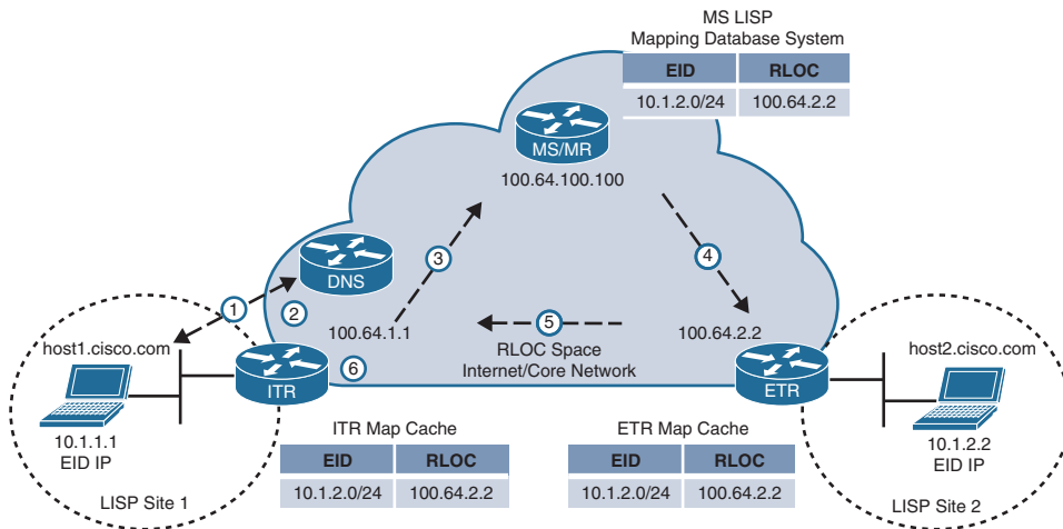
Figure 16-9 Map Request and Reply
