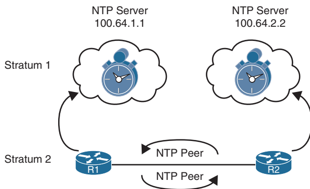
Figure 15-3 NTP Stratums
