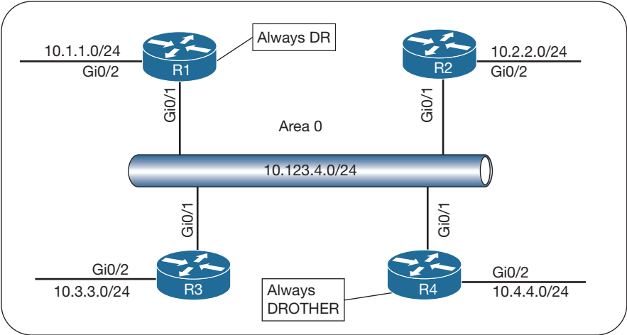
Figure 8-10 OSPF Topology for DR/BDR Placement
