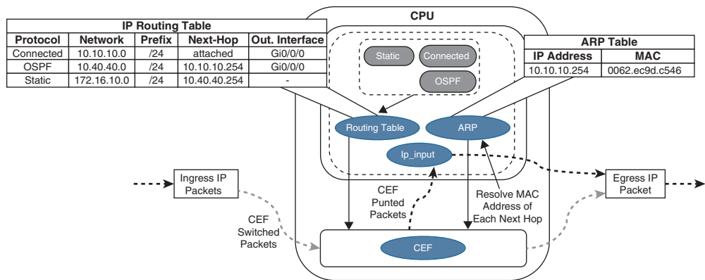
Figure 1-6 Process Switching
