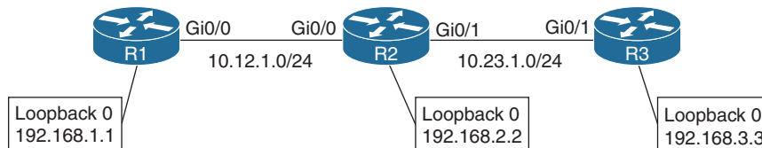
Figure 15-5 Object Tracking
