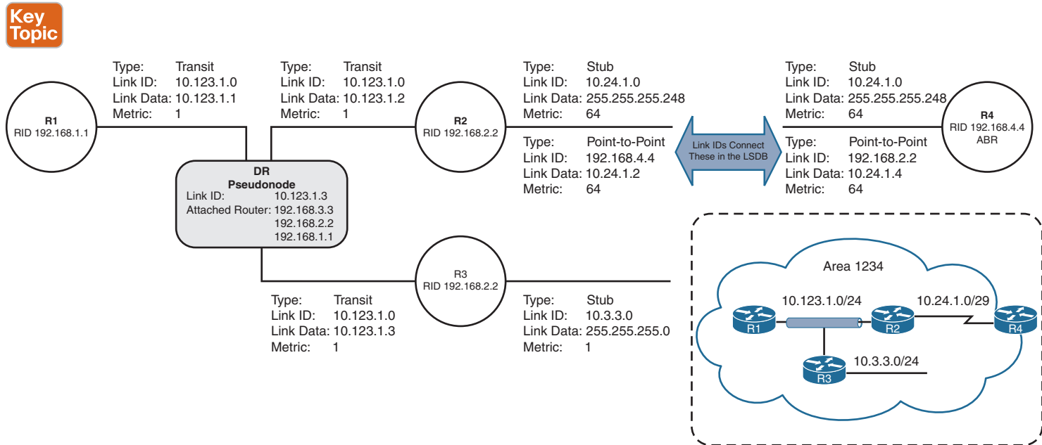
Figure 9-8 Visualization of Area 1234 with Type 1 and Type 2 LSAs
