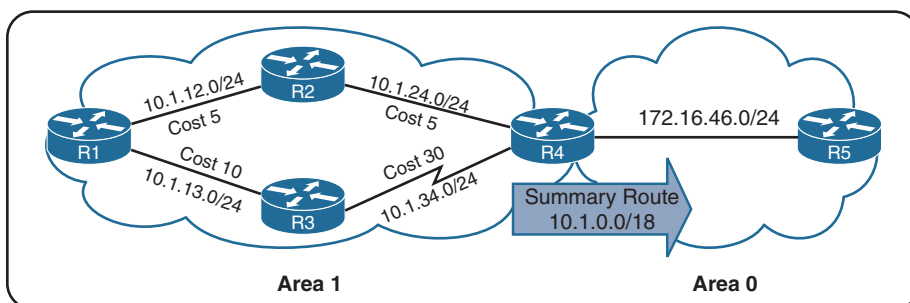
Figure 9-18 Topology Example with Summarization
