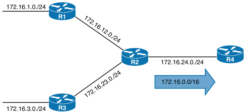
Figure 7-15 EIGRP Summarization
