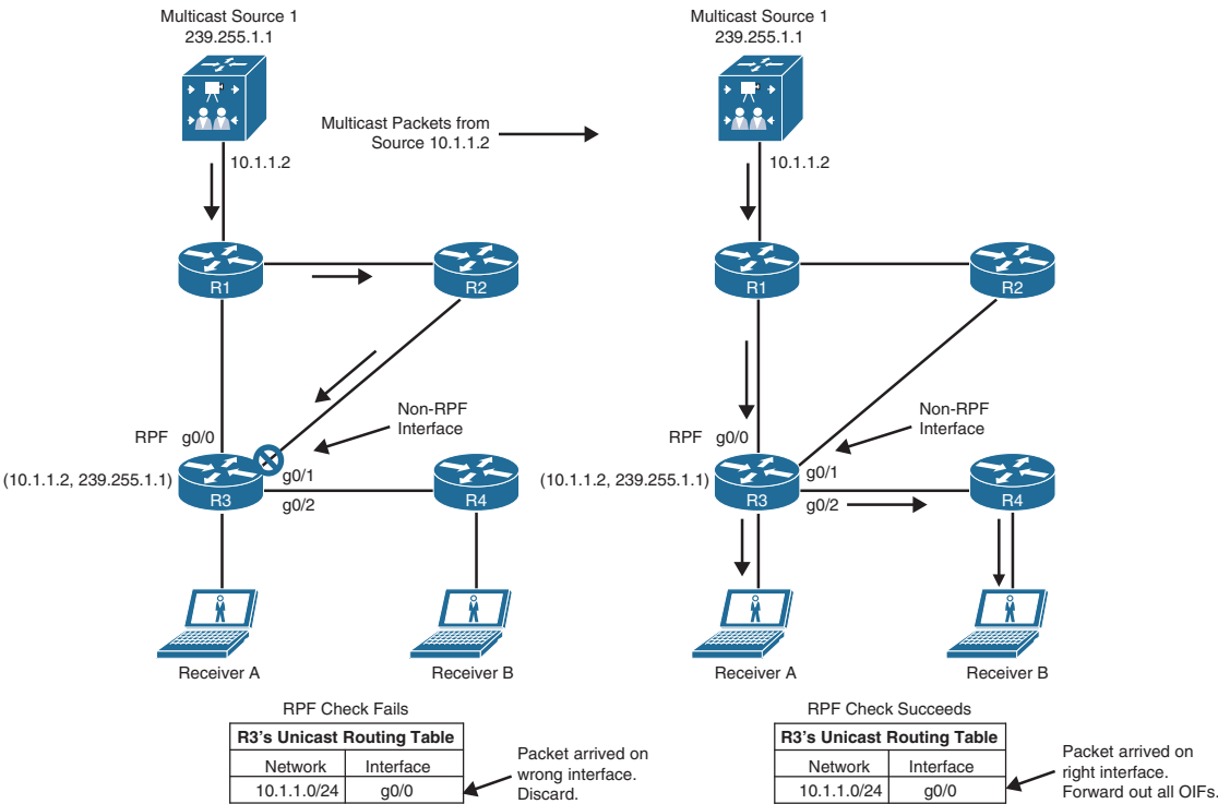
Figure 13-19 RPF Check
