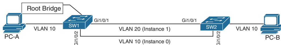
Port VLAN Assignment and VLAN-to-MSTI Mapping
