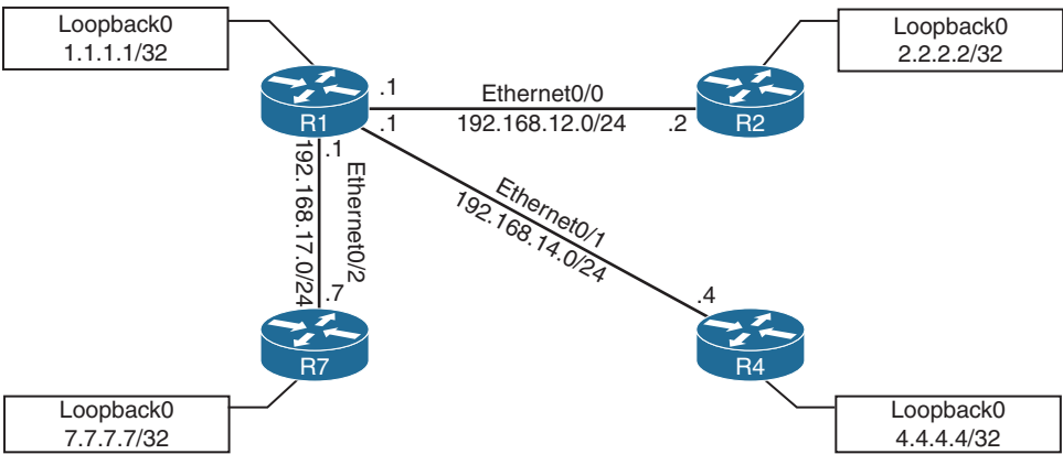
Figure 24-2 Debugging Topology
