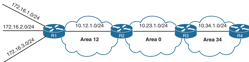
Figure 9-22 Expanded Topology for Filtering Routes
