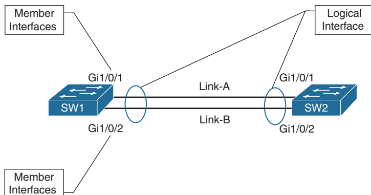
Figure 5-3 EtherChannel Components
