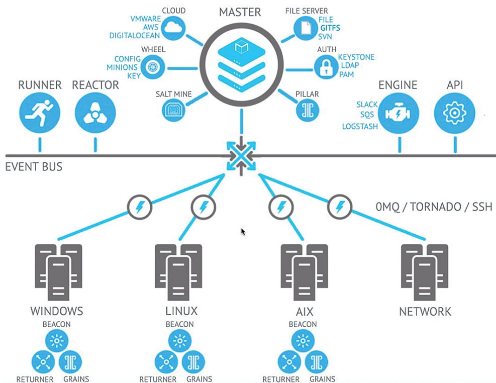
Figure 29-5 High-Level SaltStack Architecture
