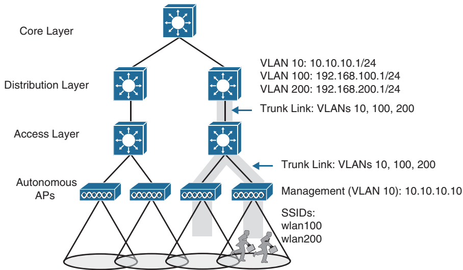
Figure 18-1 Wireless Network Topology Using Autonomous APs
