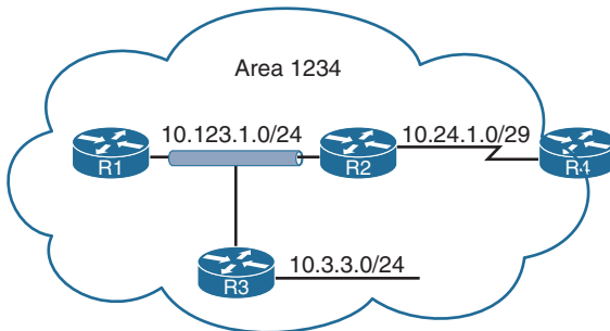
Figure 9-6 Type 1 LSA Flooding Reference Topology
