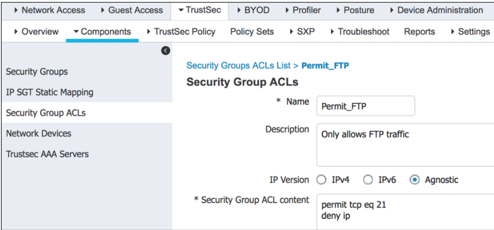
Figure 25-16 Permit FTP SGACL Contents
