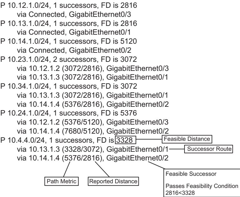
Figure 7-3 EIGRP Topology Output
