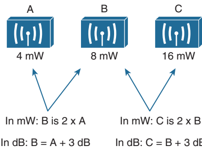
Figure 17-16 Comparing Power Levels Using dB
