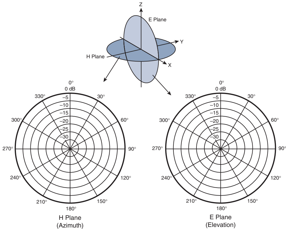
Figure 18-10 Recording an Isotropic Antenna Pattern on E and H Polar Plots
